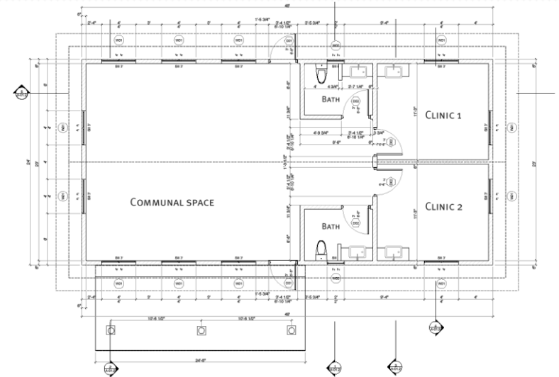
FLOOR PLAN SCALE: 1/4" = 1'-0" 1
